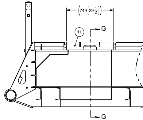
SECTION F-F
