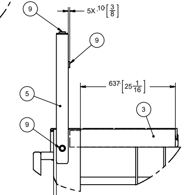
DETAIL E SCALE 1 : 8
