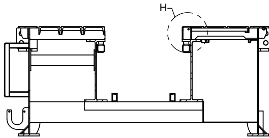
SECTION G-G
