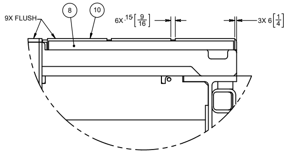
DETAIL B SCALE 1 : 4
