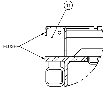
DETAIL H SCALE 1 : 3
